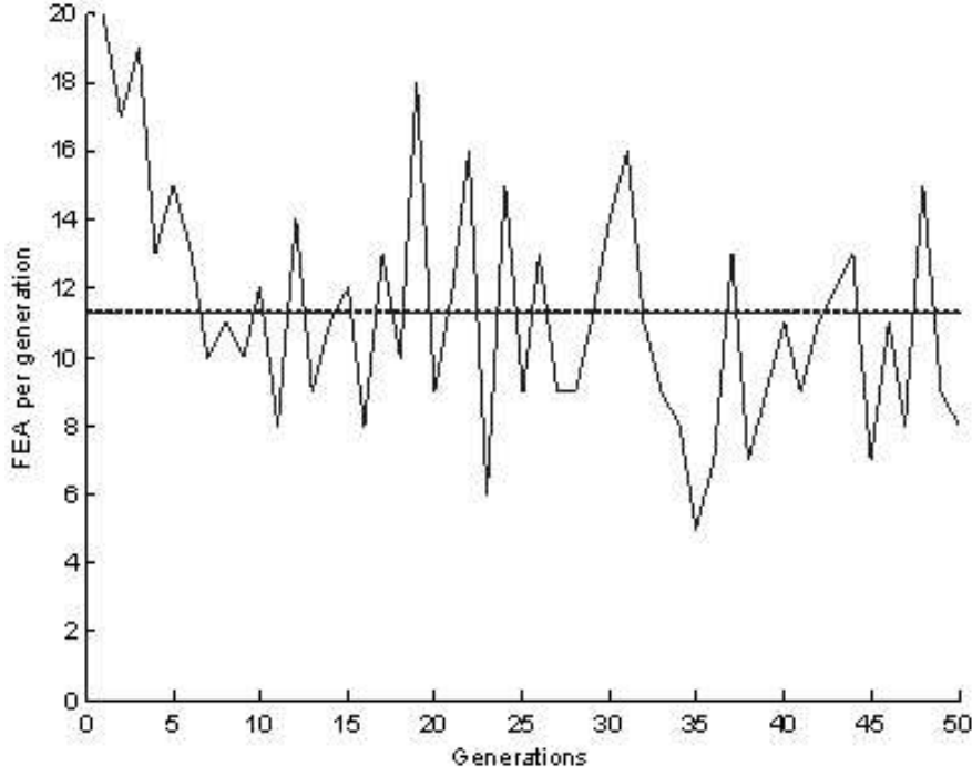
Figure 2.6: Plot of the generation number vs. number of FEA evaluations for the 2D truss frame in a single run using GA-AFFG.
