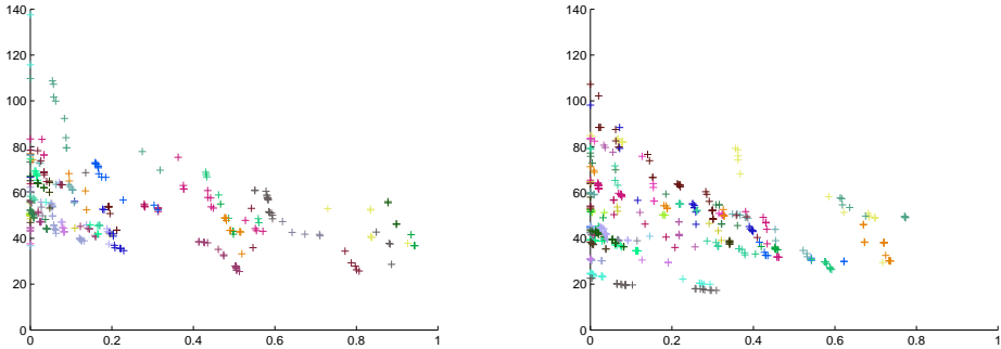
Figure 4.5: 30 independent runs of the NSGA-II (left panel) and AFG-NSGA-II (right panel) for the ZDT4 test problem using 1,000 real fitness function evaluations.
