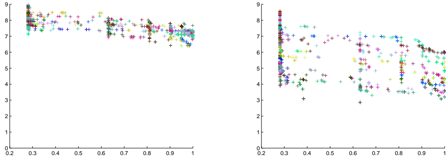
Figure 4.6: 30 independent runs of the NSGA-II (left panel) and AFG-NSGA-II (right panel) for the ZDT6 test problem using 1,000 real fitness function evaluations.
