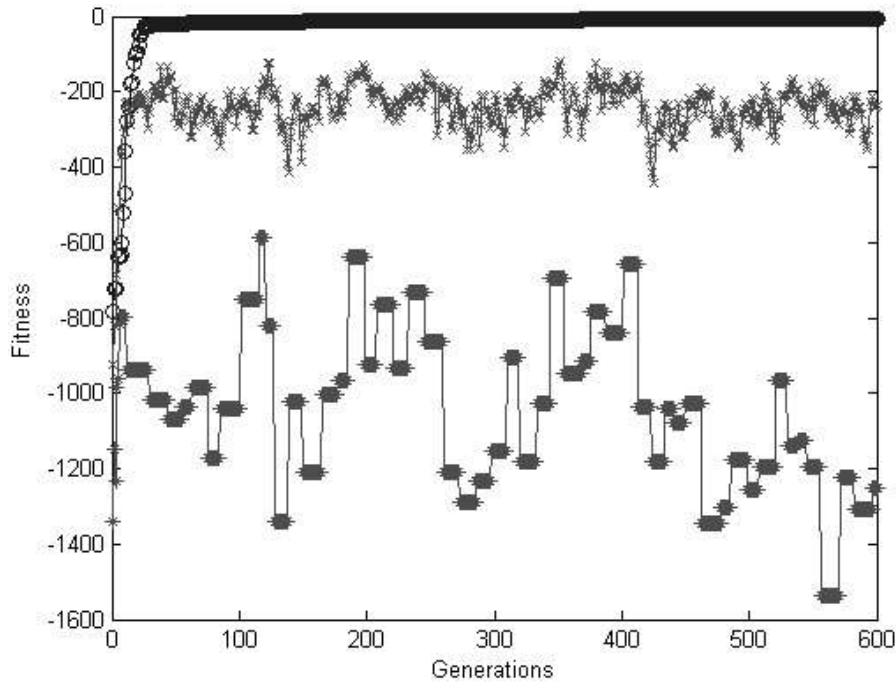
Figure 2.9: Generation number vs. fitness for the piezoelectric actuator using our proposed GA-AFFG for a single run: best (circle), average (cross) and worst (asterisk) of individuals at each generation.
