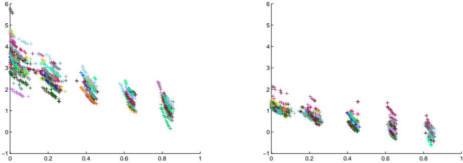
Figure 4.4: 30 independent runs of the NSGA-II (left panel) and AFG-NSGA-II (right panel) for the ZDT3 test problem using 1,000 real fitness function evaluations.
